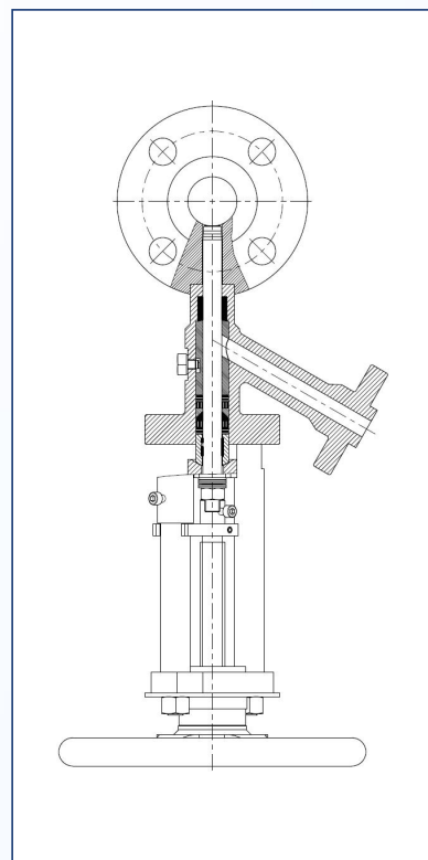
软密封带放净环
