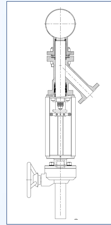
带适配管道柱塞阀 (可拆卸适配管道)
